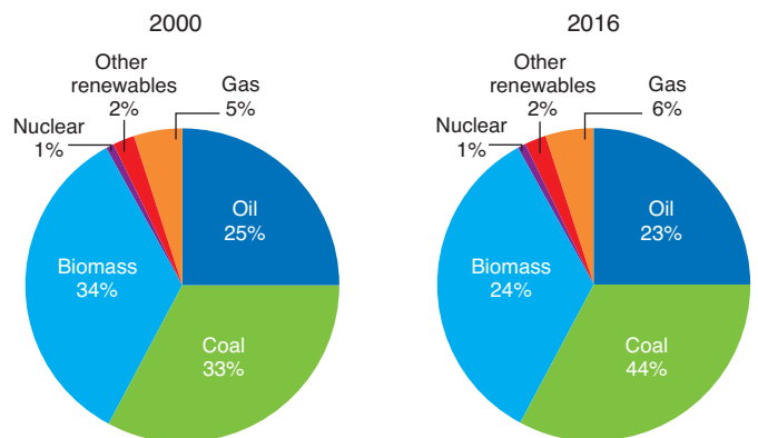
Fig. 6 – Primary energy consumption by energy type 8
