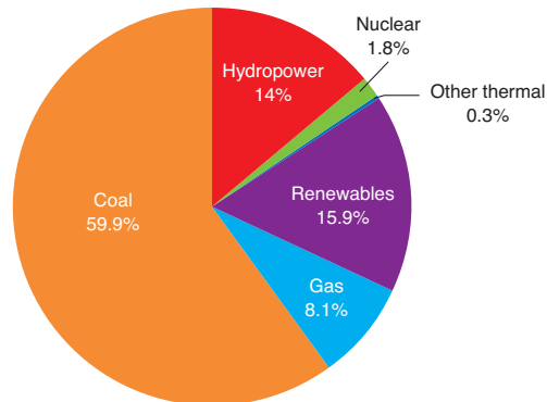
Fig. 5 – Power capacity installed in 2017
