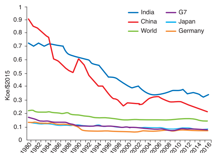
Fig. 12 – Energy intensity of industry in various countries (in koe/$2015)
